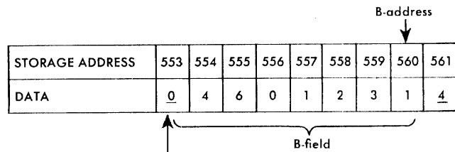
Figure 10. Data and Instruction Addressing
