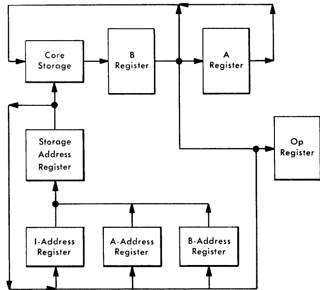
Figure 11. Processing Unit Registers
