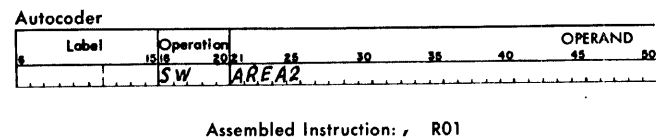
Figure 47. Set Word Mark (One Address)
