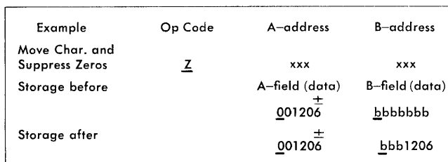
Figure 38. Move Characters and Suppress Zeros Operation Example
