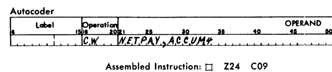
Figure 48. Clear Word Mark (Two Addresses)
