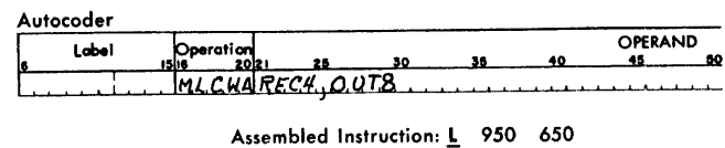
Figure 44. Load Characters to A Word Mark (Two Fields)
