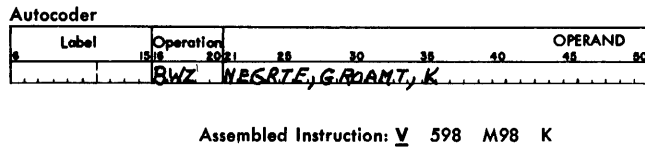
Figure 34. Branch if Word Mark and/or Zone
