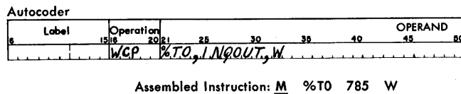
Figure 63. Write on 1447 Console
