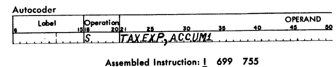
Figure 27. Zero and Subtract (Two Fields)
