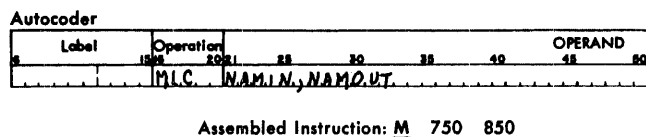
Figure 36. Move Characters to A or B Word Mark (Two Fields)
