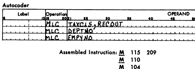
Figure 37. Move Characters to A or B Word Mark (One Field)
