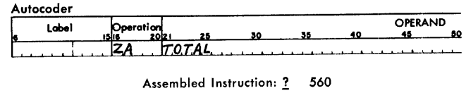
Figure 26. Zero and Add (One Field)
