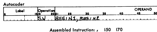
Figure 46. Set Word Mark (Two Addresses)
