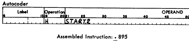
Figure 54. Halt and Branch
