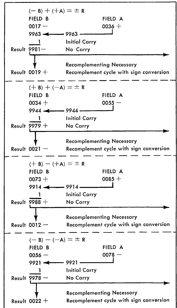
Figure 20. Complement-Add (with Recomplementing) Cycle Examples
